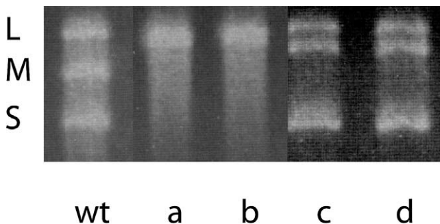
Fig. 9. dsRNA isolated from wild-type \phi 8 (wt); from two-segment virus containing normal L and the SM chimeric segment (a, b); and from three-segment virus containing normal L and S and a truncated chimeric MS segment (c, d).
